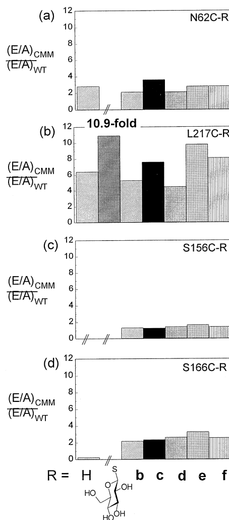
Figure 3. E/A of deprotected glyco-CMMs relative to WT. A break in the axis indicates that the value was not determined. Glycosylation with deprotected reagents 1b–f increases the E/A ratio in all cases. The greatest effects are observed at positions 62, in the S 2 pocket (a), and 217, in the S 1 ' pocket (b), where the largest increases in E/A result in values up to 10.9-fold greater than WT. At both sites E/A is higher for the β-linked glyco-CMMs than the α-linked ones. At positions 156, (c) and 166 (d), in the S 1 pocket, there is little variation in E/A .
