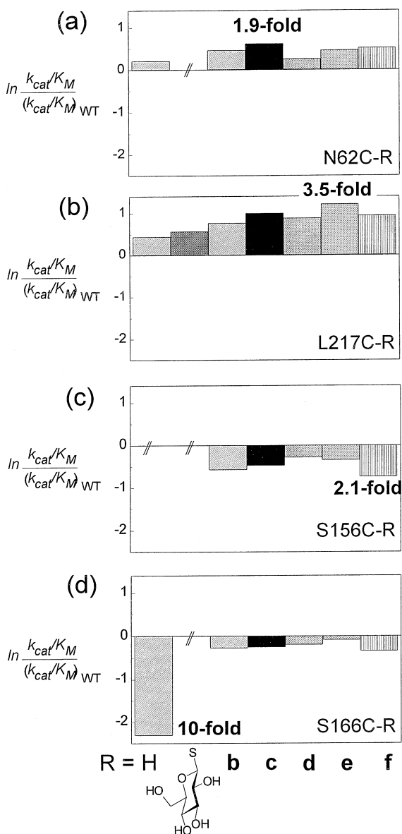
Figure 1. Esterase k_{cat}/K_M s for deprotected glyco-CMMs relative to WT. (a) At position 62, in the S_1 pocket, glycosylation leads to a series of enzymes that have similar activities that are 1.3- to 1.9-fold greater than WT. (b) At position 217, in the S_1' pocket, glycosylation also increases k_{cat}/K_M , to a maximum 3.5-fold greater than WT for L217C-S-Et- \beta -Glc (-e). (c) At position 156, in the S_1 pocket, glycosylation leads to reduction in k_{cat}/K_M . (d) At position 166, in the S_1 pocket, the dramatic loss of activity upon mutation to cysteine ( R = H ) is restored by glycosylation. All five S166C deprotected glyco-CMMs have similar k_{cat}/K_M s that are 1.1- to 1.4-fold lower than WT.
